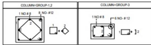
SCHEDULE OF R.C.C COLUMN & FOOTINGS
